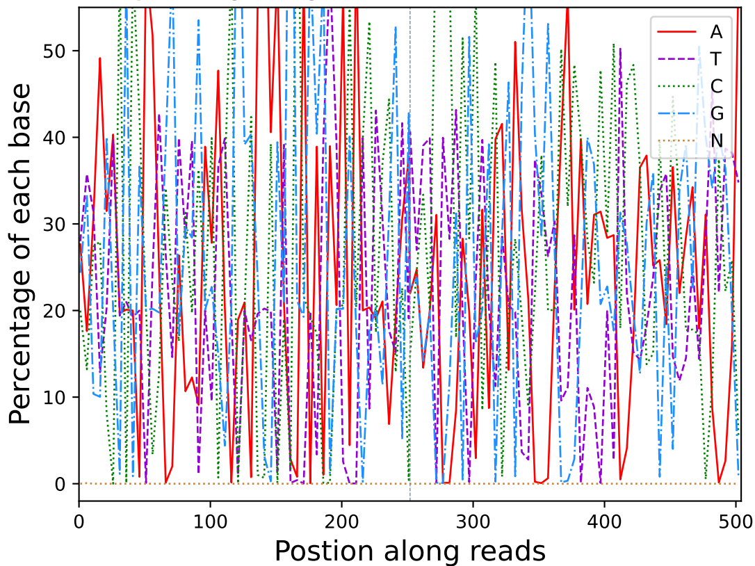
Base percentage along reads (R10612)
